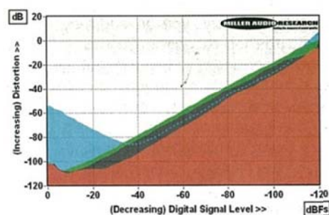
ABOVE: THD vs. digital level over 120dB. S/PDIF input (48kHz/24-bit; 1kHz, red); CD (1kHz, black); USB (1kHz, green); S/PDIF (1kHz, tube output, blue)
